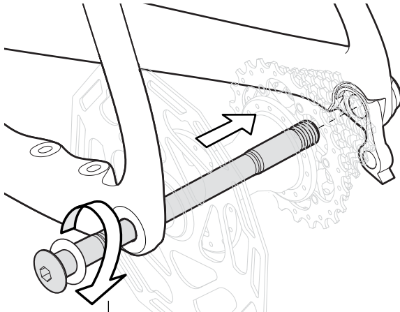
Ensure thru-axle washer is present for installation.
