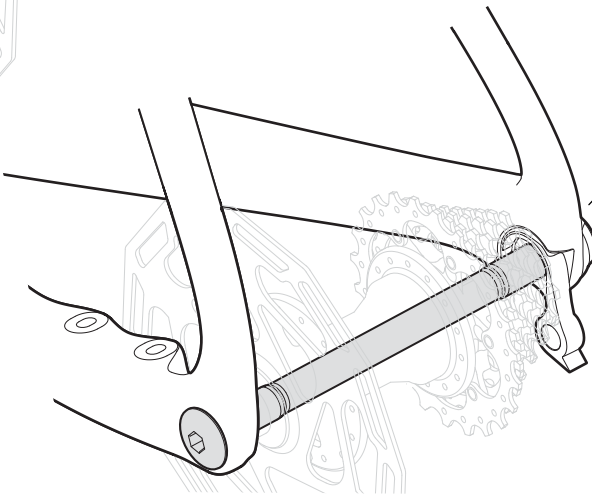
Tighten front axle to 12-15 N·m.
